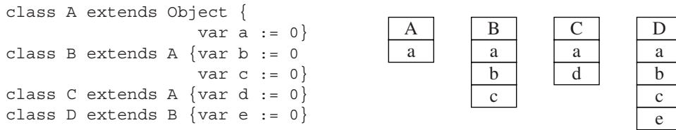
FIGURE 14.2. Single inheritance of data fields.
