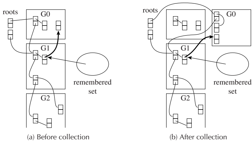
FIGURE 13.12. Generational collection. The bold arrow is one of the rare pointers from an older generation to a newer one.
