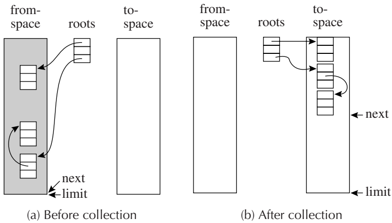
FIGURE 13.7. Copying collection.
